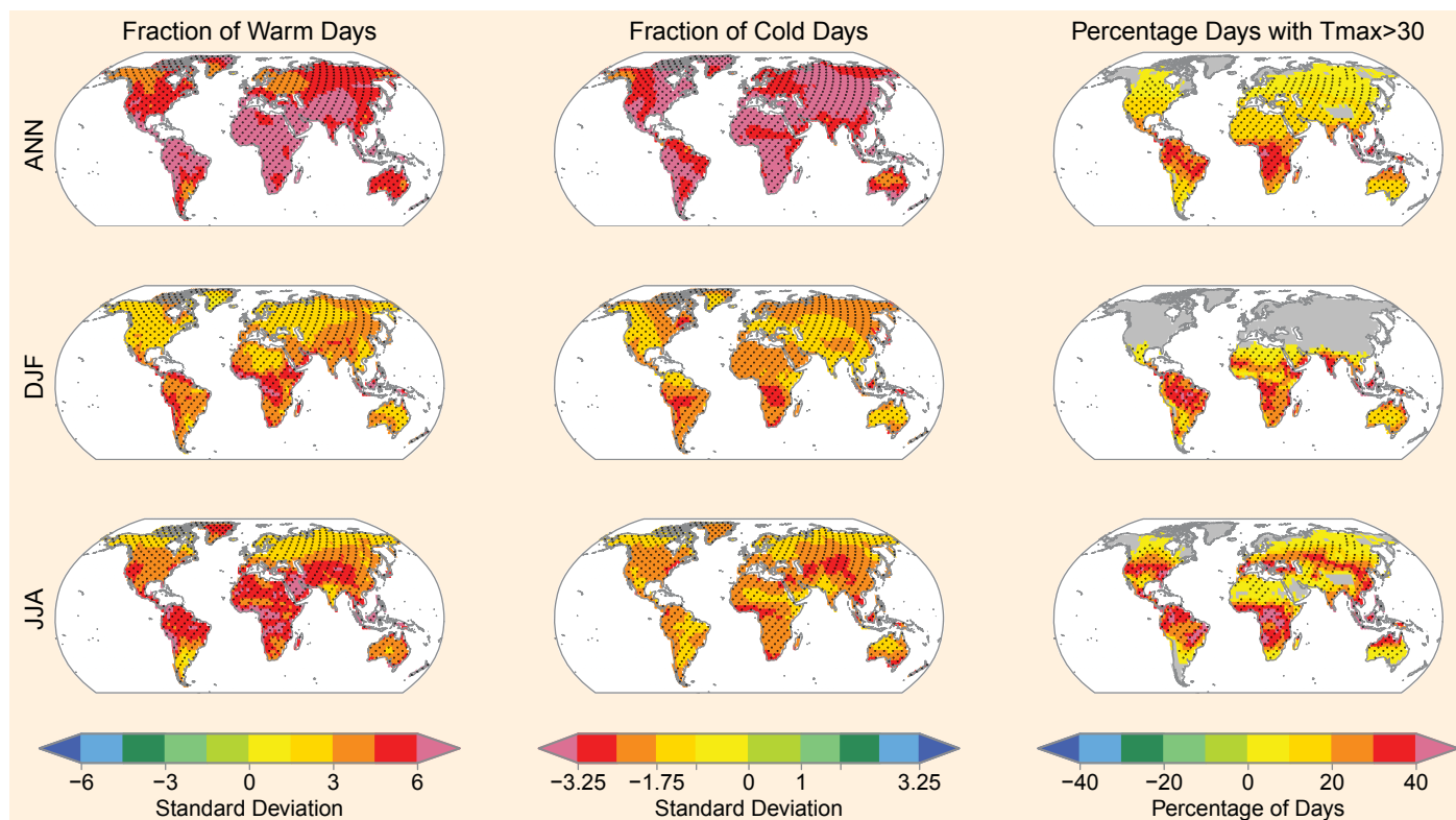
Figure 3-3 | Projected annual and seasonal changes in three indices for daily T_{max} for 2081-2100 with respect to 1980-1999, based on 14 GCMs contributing to the CMIP3. Left column: fraction of warm days (days in which T_{max} exceeds the 90th percentile of that day of the year, calculated from the 1961-1990 reference period); middle column: fraction of cold days (days in which T_{max} is lower than the 10th percentile of that day of the year, calculated from the 1961-1990 reference period); right column: percentage of days with T_{max} > 30^{\circ}\text{C} . The changes are computed for the annual time scale (top row) and two seasons (December-January-February, DJF, middle row, and June-July-August, JJA, bottom row) as the fractions/percentages in the 2081-2100 period (based on simulations for emission scenario SRES A2) minus the fractions/percentages of the 1980-1999 period (from corresponding simulations for the 20th century). Warm day and cold day changes are expressed in units of standard deviations, derived from detrended per year annual or seasonal estimates, respectively, from the three 20-year periods 1980-1999, 2046-2065, and 2081-2100 pooled together. T_{max} > 30^{\circ}\text{C} changes are given directly as differences in percentage points. Color shading is only applied for areas where at least 66% (i.e., 10 out of 14) of the GCMs agree on the sign of the change; stippling is applied for regions where at least 90% (i.e., 13 out of 14) of the GCMs agree on the sign of the change. Adapted from Orłowsky and Seneviratne (2011); updating Tebaldi et al. (2006) for additional number of indices and CMIP3 models, and including seasonal time frames. For more details, see Appendix 3.A.
