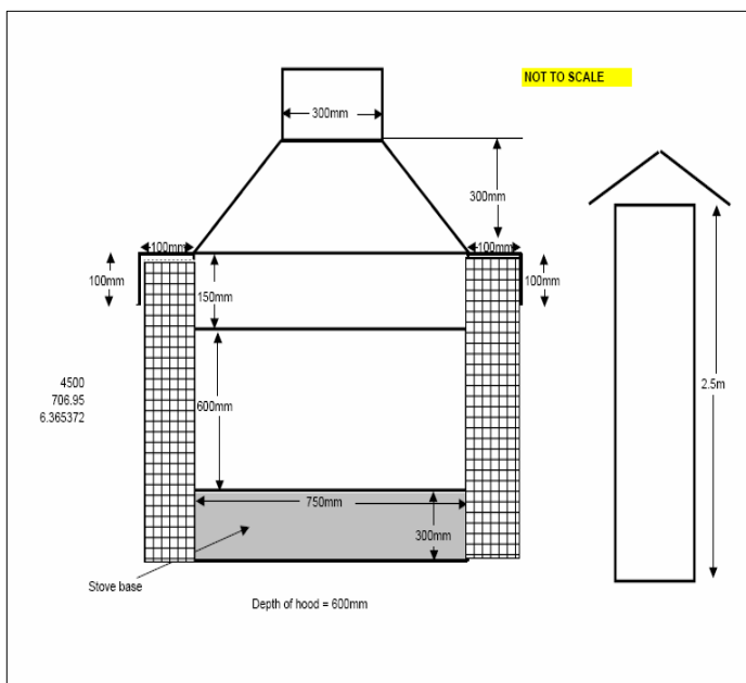
Figure 5: Stove dimensions used in the Tanzania smoke hood.
