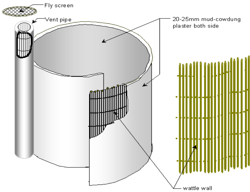
Spiral superstructure
