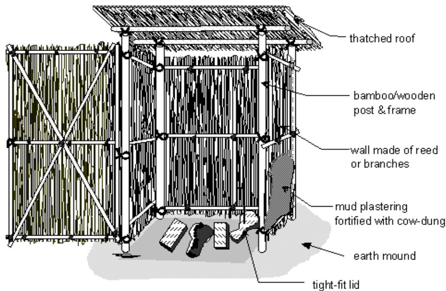
low-cost superstructure
